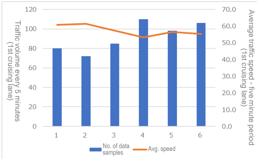
[Traffic volume and speed of 1st cruising lane (CD section)]
