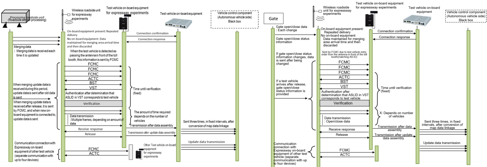
Fig. Transmission sequence between units when providing ETC gate passing support
