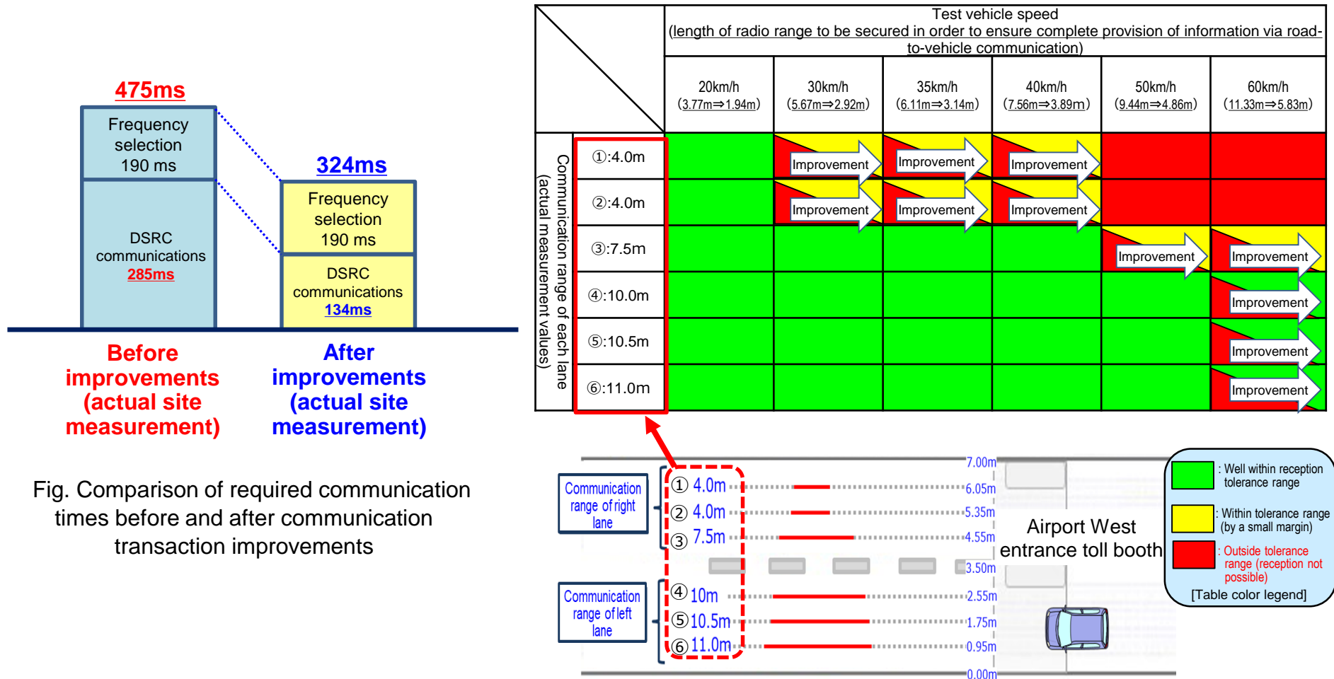
Fig. Evaluation of vehicle driving speed tolerance within radio range
