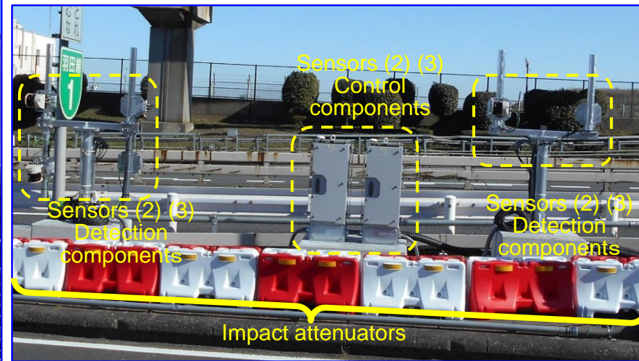
Figure 3-3 Sensors (2) (3) installation and appearance of impact attenuators
