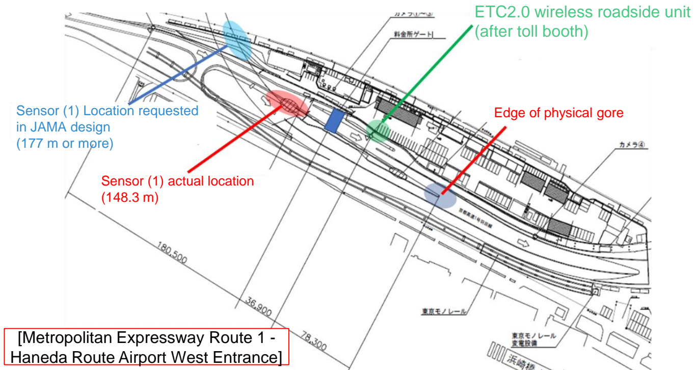
Fig. Comparison of roadside sensor locations requested in JAMA design and actual installation locations
