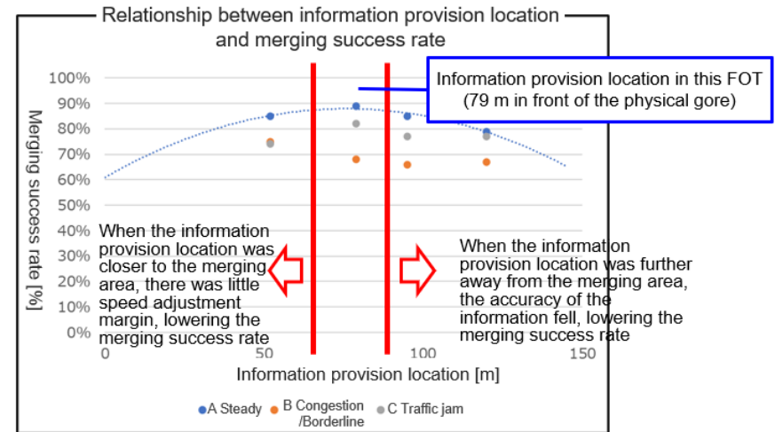
Merging success rates by roadside unit, sensor location, and cruising line traffic conditions
