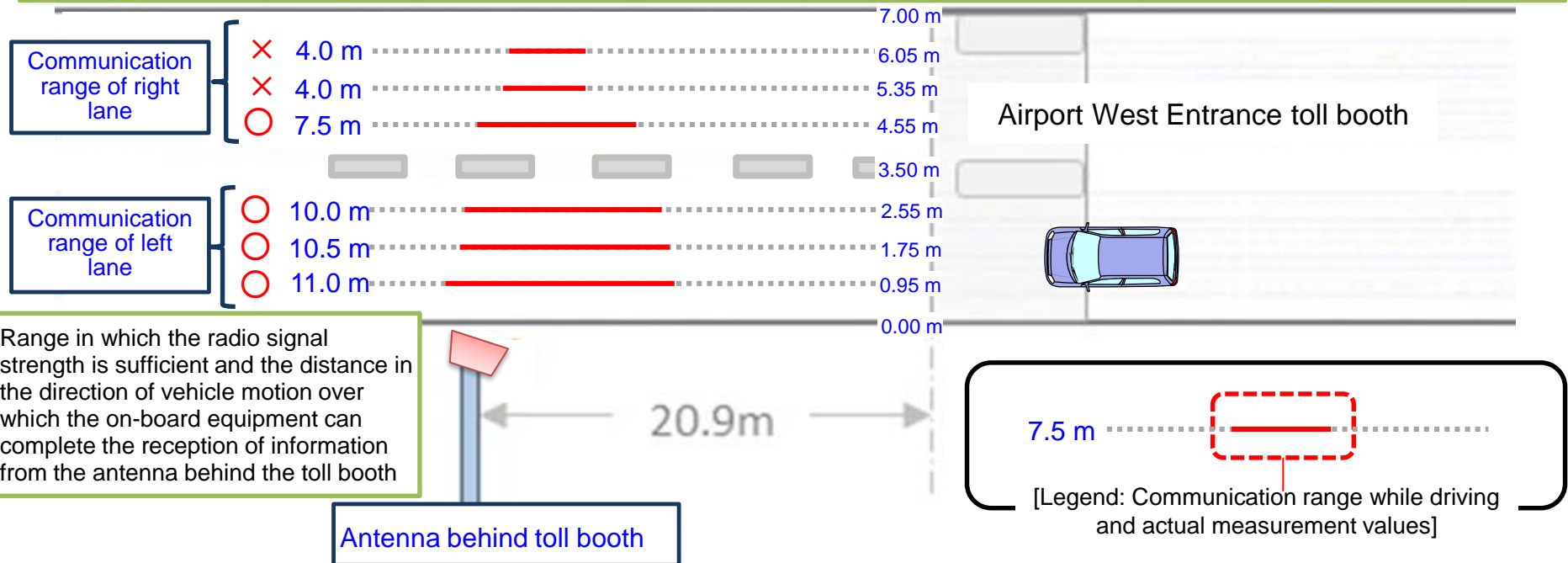
Fig. Antenna behind toll booth - Range of possible communication range by location in lane [for envisioned speed of 30 km/h]
