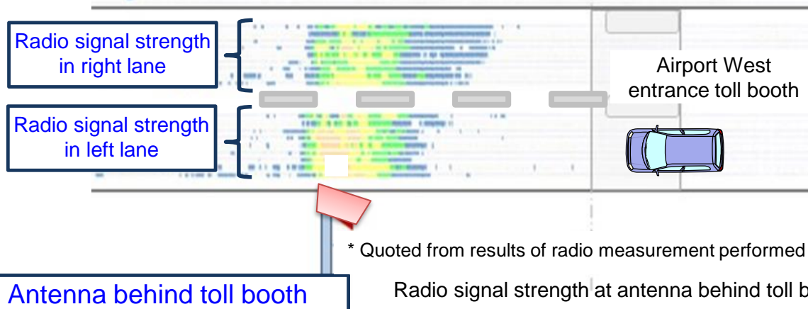
Radio signal strength at antenna behind toll booth (actual measurement values: schematic diagram)
